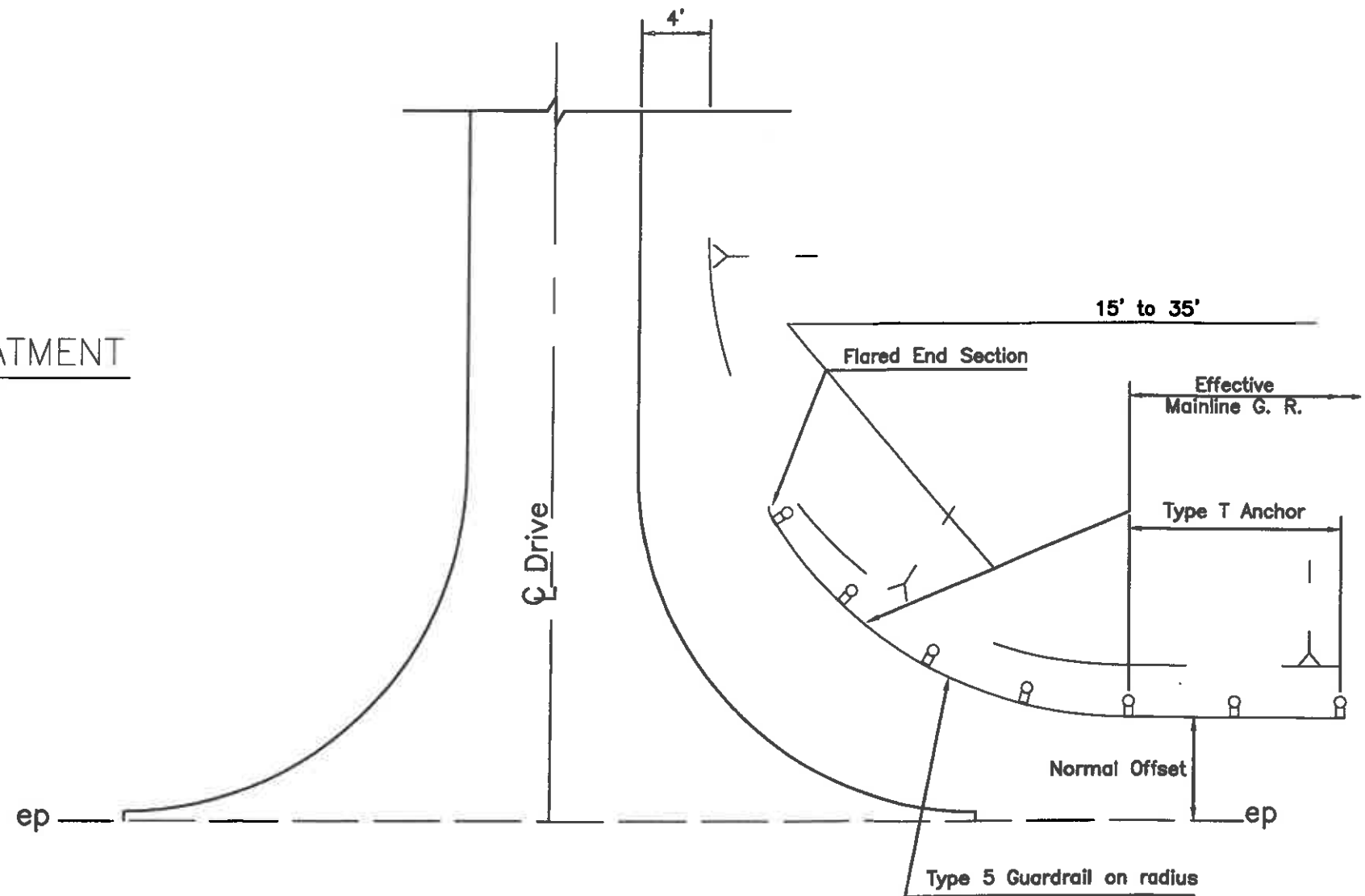
TYPICAL DRIVEWAY OPENING TREATMENT
