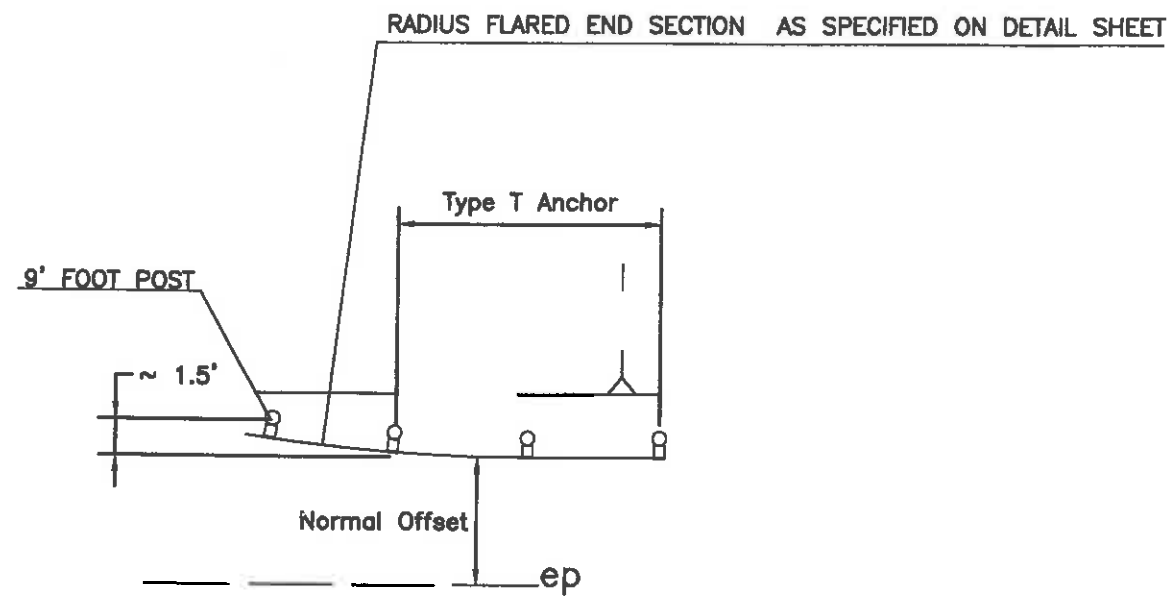
TYPE T ANCHOR ASSEMBLY, MODIFIED END TREATMENT
